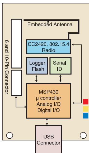
TPR2400CA Block Diagram
